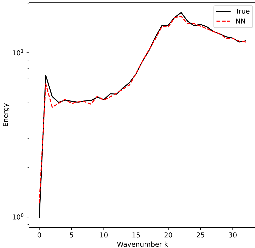
1D Spectrum Space
